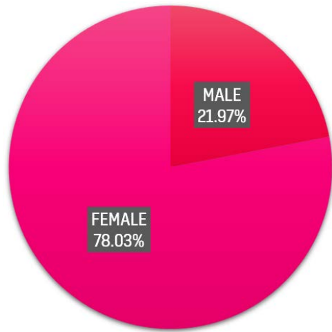
LOWER QUARTILE
